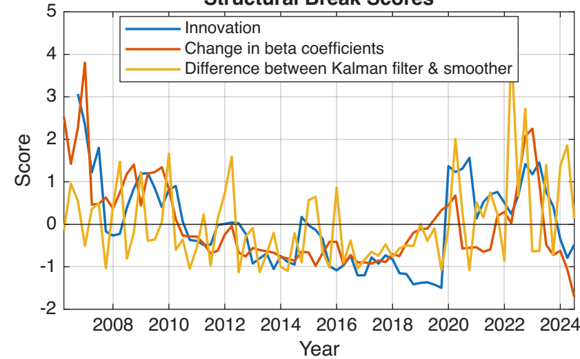
Structural Break Scores
