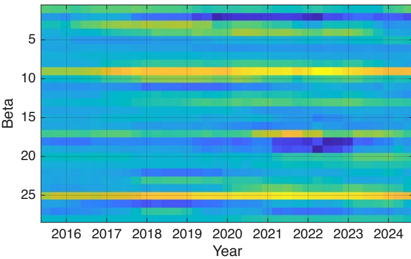
Kalman Filter
