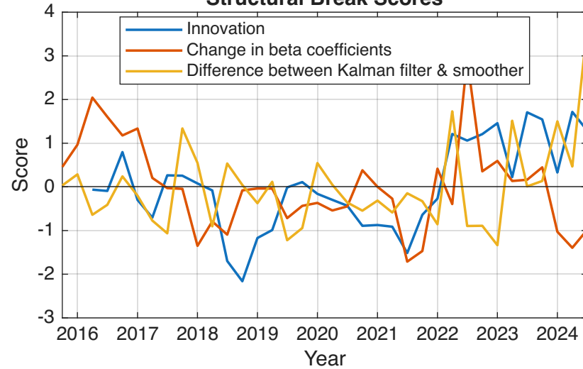
Structural Break Scores
