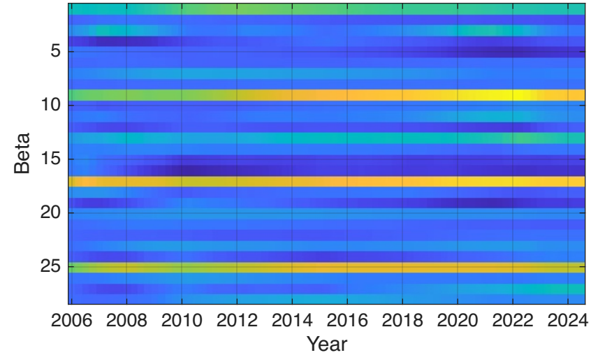
Kalman Smoother
